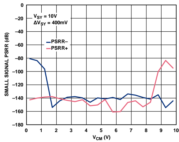
Figure 17. Small Signal PSRR vs. Common-Mode Voltage
