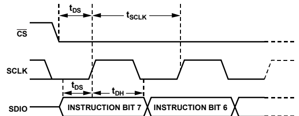
Figure 126. Timing Diagram for an SPI Register Write
