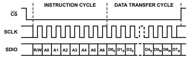
Figure 124. Serial Register Interface Timing, LSB-First Write
