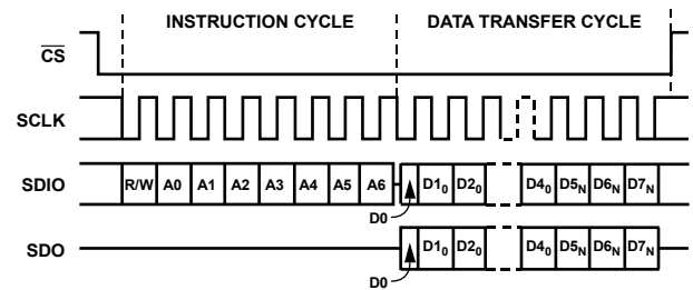
Figure 125. Serial Register Interface Timing, LSB-First Read
