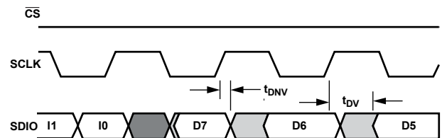
Figure 127. Timing Diagram for an SPI Register Read
