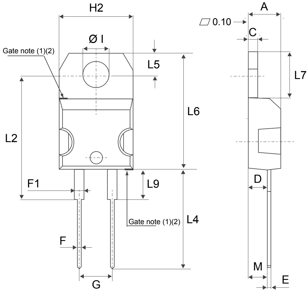
Figure 14. TO-220AC package outline
