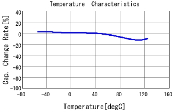
■ RDER73A104K5B1H03B C-Temp. capchange, DCOV, AC1Vrms
