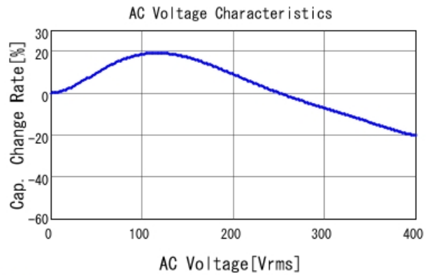
■ RDER73A104K5B1H03B C-AC Voltage capchange, DC0V, 25.0
