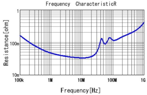
■ RDER73A104K5B1H03B R DC0V, 25degC
