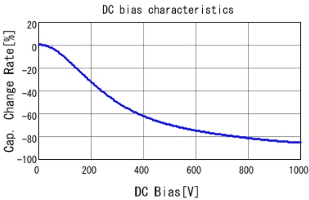
■ RDER73A104K5B1H03B C-DC bias capchange, 25.0degC, AC1
