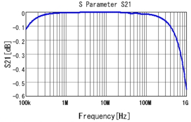
■ RDER73A104K5B1H03B S21 DCOV, 25degC
