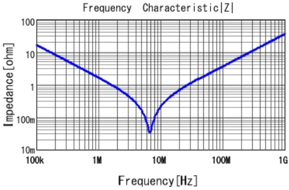
■ RDER73A104K5B1H03B |Z| DC0V, 25degC
