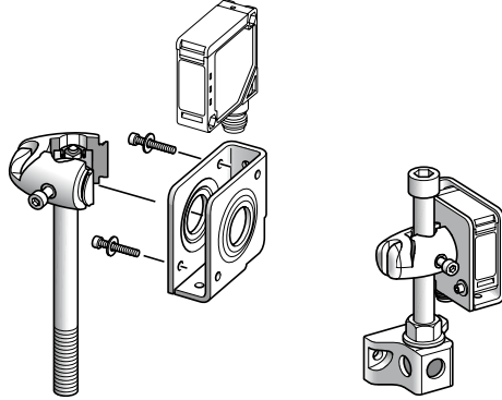
Mounting example
