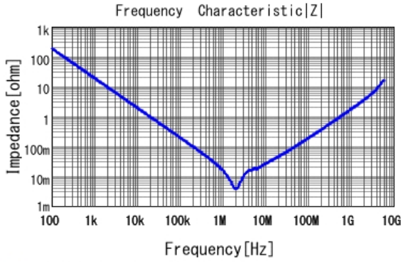
■ GRM21BR61C106ME15 |Z| DCOV, 25degC
