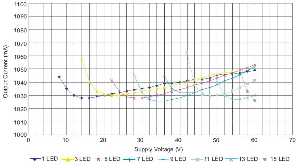
ZXLD1362 Output Current L = 150 \mu H
