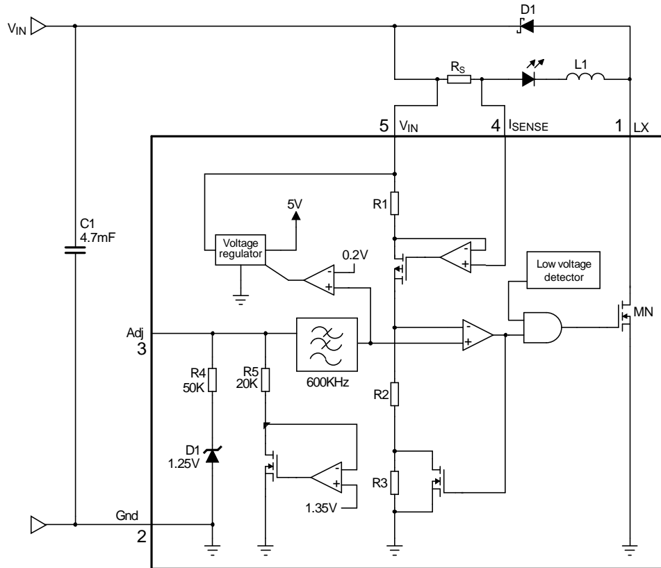
Figure 1. Block Diagram
