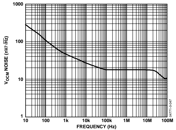
Figure 35. V_{OCM} Voltage Noise vs. Frequency
