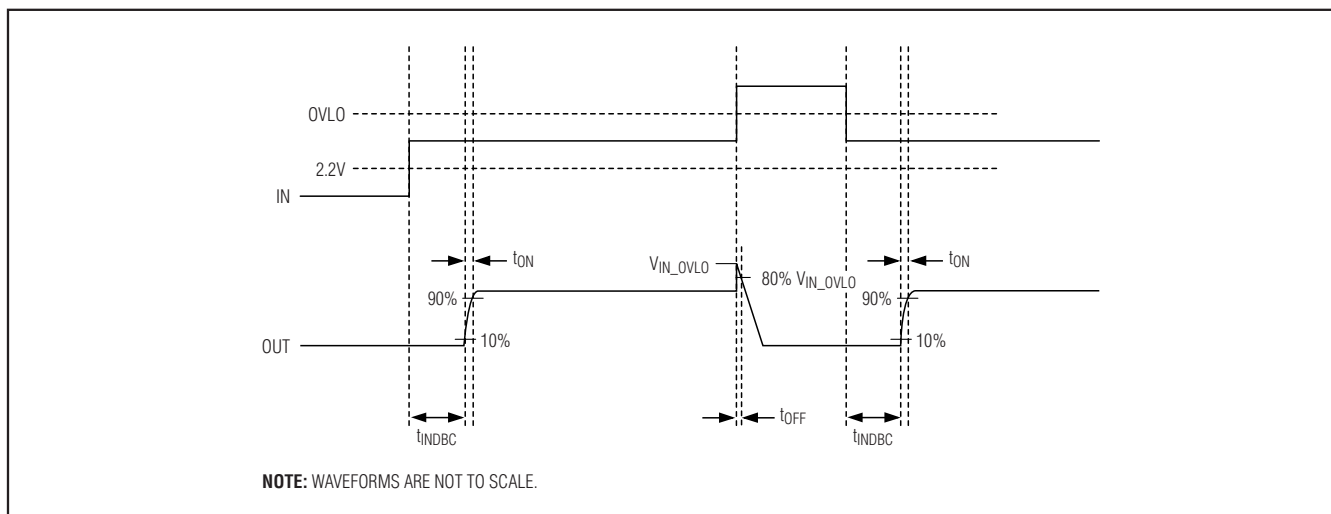
Figure 1. Timing Characteristics
