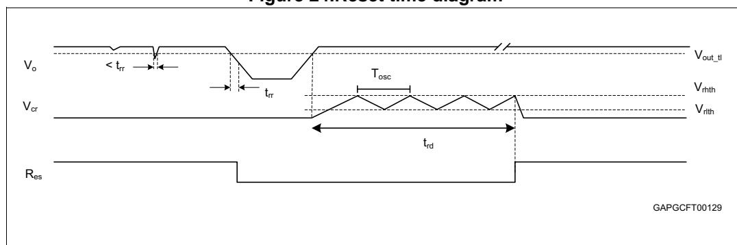
Figure 24.Reset time diagram
