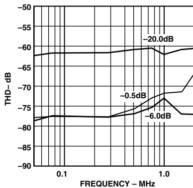
TPC 7. THD vs. Input Frequency (Input Span = 5.0 V p-p, V_{\text{CM}} = 2.5 \text{ V} )
