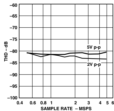
TPC 17. THD vs. Sample Rate ( A_{IN} = -0.5 dB, f_{IN} = 500 kHz, V_{CM} = 2.5 V)
