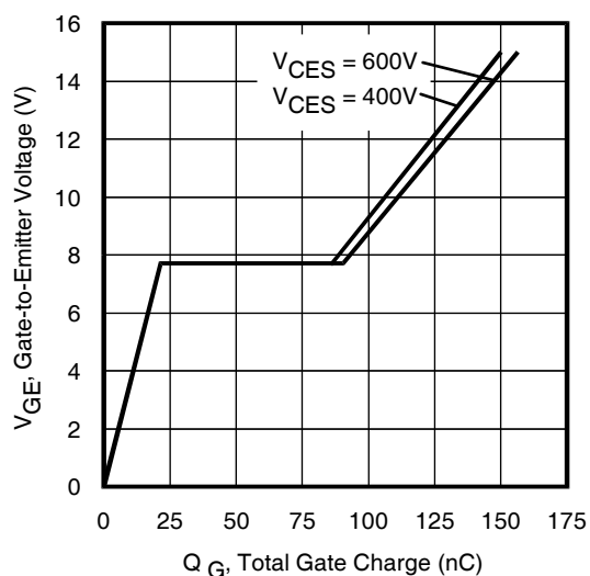
Fig. 18 - Typical Gate Charge vs. V_{GE} I_{CE} = 30A ; L = 600\mu H
