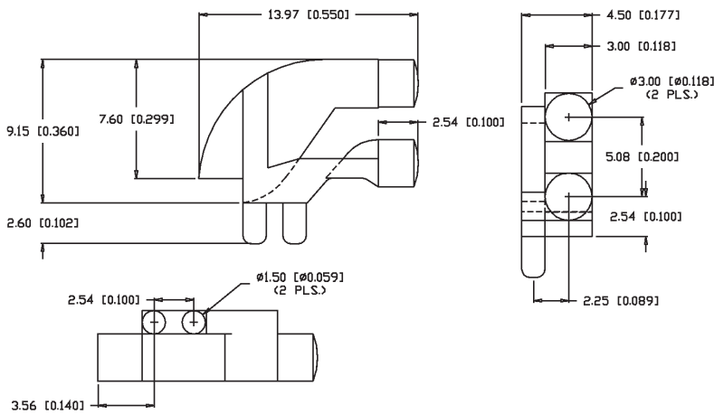
Figure 12 Part # LPF-C011302S
