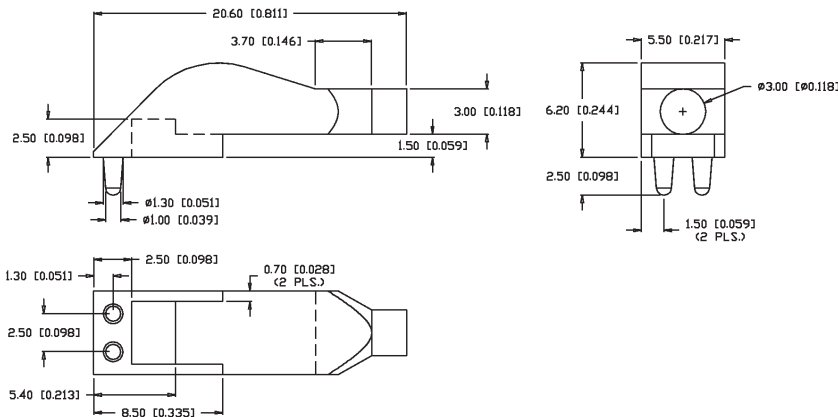
Figure 12 Part # LPF-C011302S
