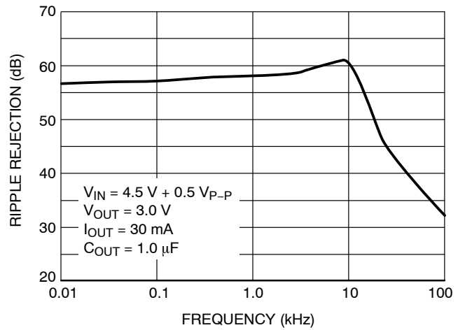
Figure 7. Ripple Rejection/Frequency
