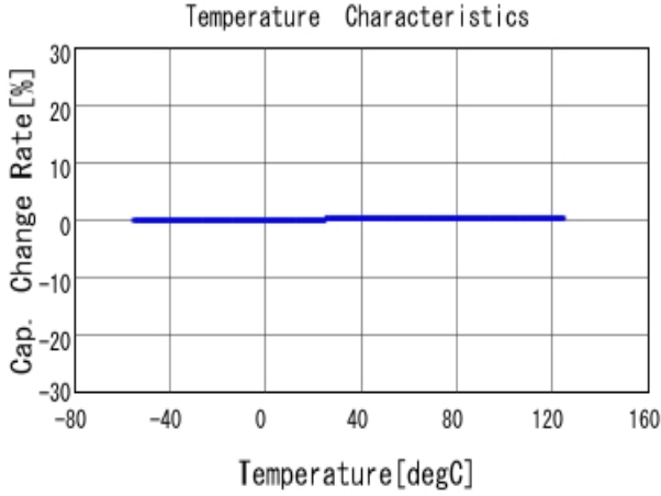
GJM1555C1H120JB01 C-Temp. capchange, DCOV, AC1Vrms
