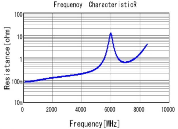
■ GJM1555C1H120JB01 R DCOV, 25degC
