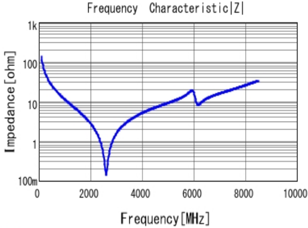
■ GJM1555C1H120JB01 |Z| DCOV, 25degC
