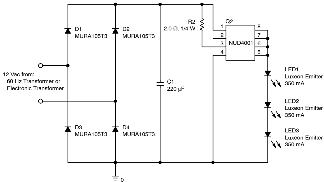
Figure 10. 12 Vac landscape lighting application circuit using the NUD4001 device to drive three 350 mA LEDs.
