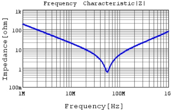
DE1E3KX102MA4BN01F |Z| DCOV, 20degC
