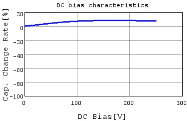
DE1E3KX102MA4BN01F C-DC bias capchange, 20.0
