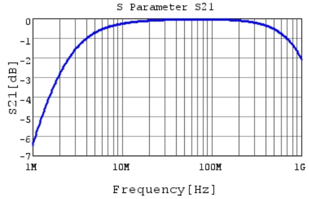
DE1E3KX102MA4BN01F S21 DCOV, 20degC
