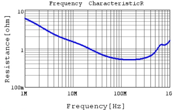
DE1E3KX102MA4BN01F R DCOV, 20degC
