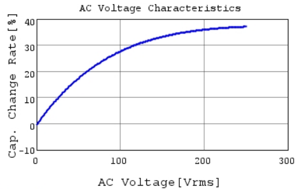
DE1E3KX102MA4BN01F C-AC Voltage capchange, I
