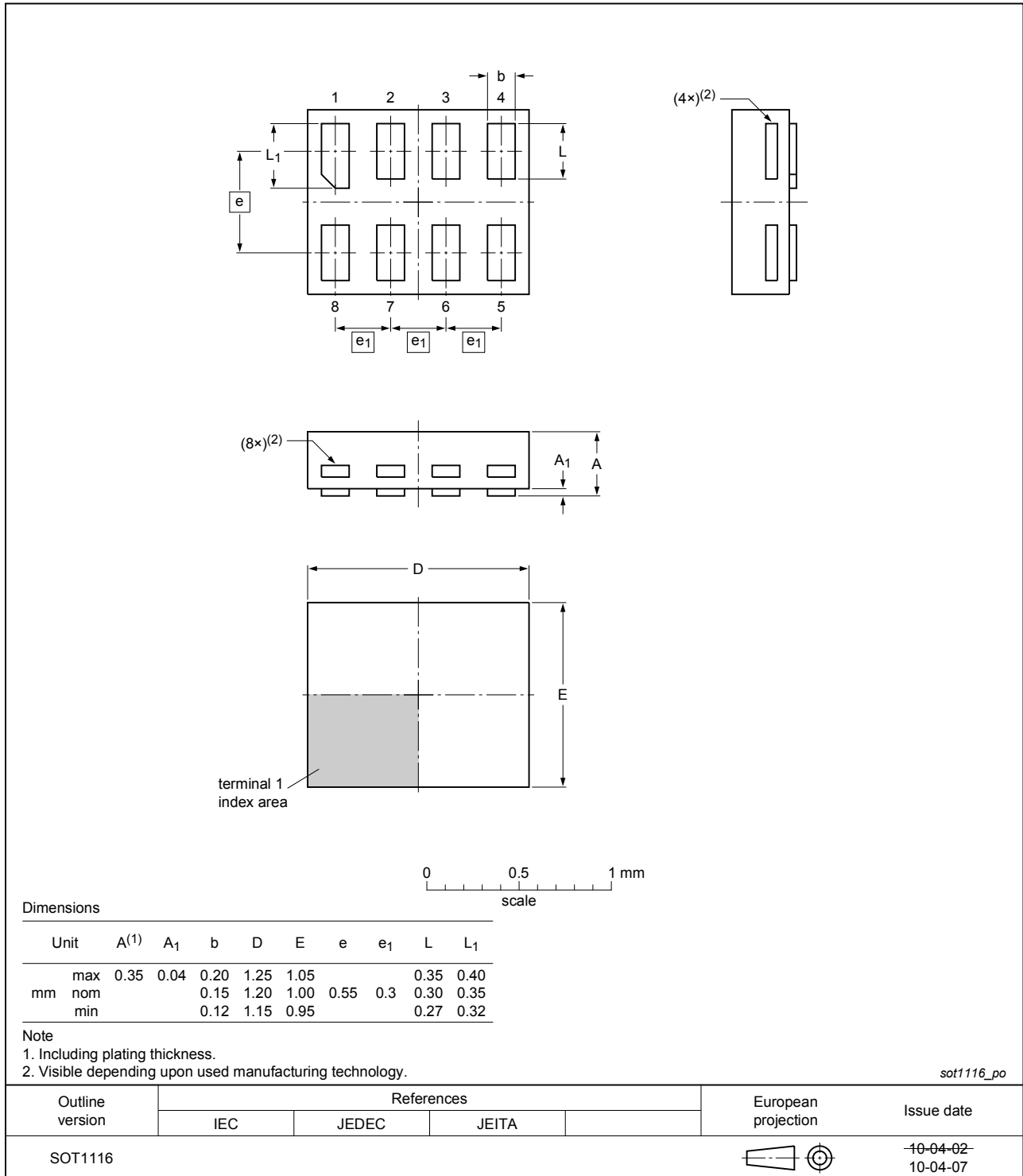
Fig. 32. Package outline SOT1116 (XSON8)
