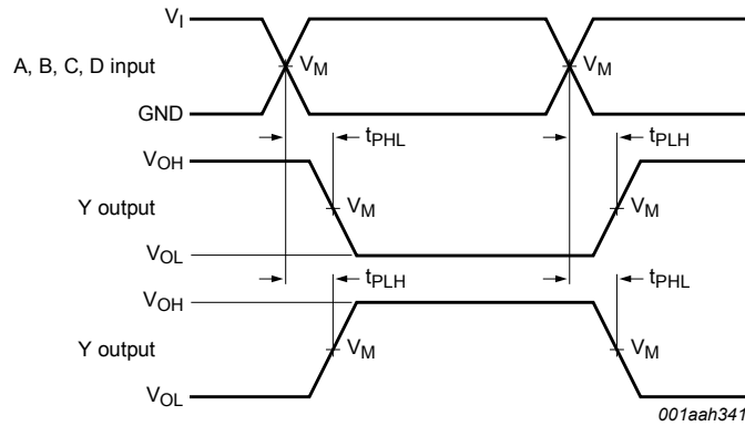
Fig. 25. The data input (A, B, C, D) to output (Y) propagation delays
