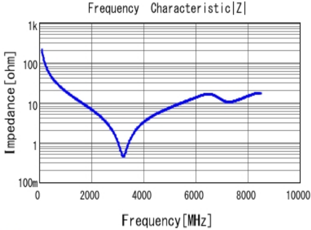
■ GRM1555C1H7R5CA01 |Z| DCOV, 25degC
