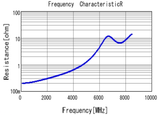
■ GRM1555C1H7R5CA01 R DCOV, 25degC
