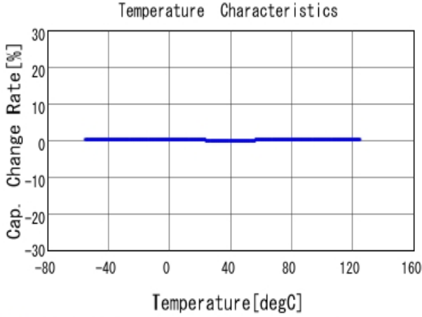
■ GRM1555C1H7R5CA01 C-Temp. capchange, DCOV, AC1Vrms
