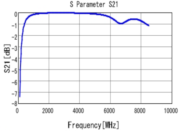
■ GRM1555C1H7R5CA01 S21 DCOV, 25degC
