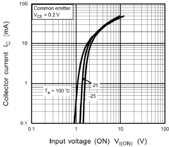
Fig. 11.1 RN1101MFV I_C - V_{I(ON)}
