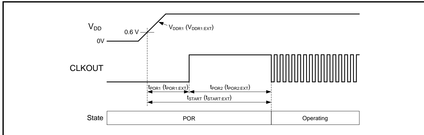
Power On AC Electrical Characteristics:
