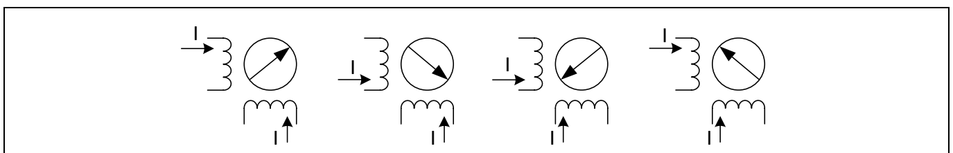
Figure 4 Full step control
