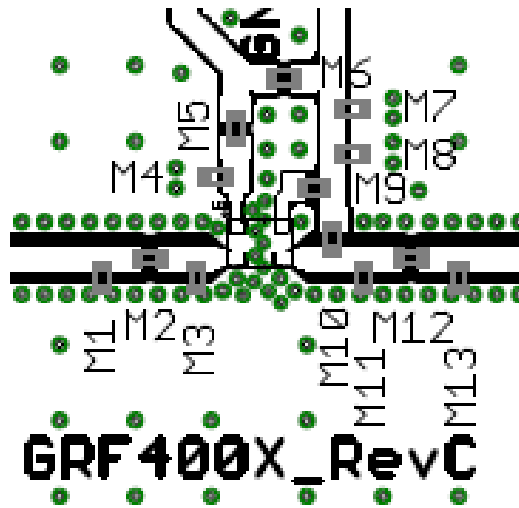
GRF1201W Evaluation Board Assembly Drawing
