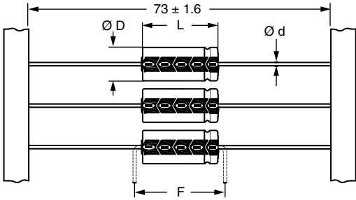
Form BR: Taped on reel Case \text{Ø D} \times \text{L} = 8 \text{ mm} \times 18 \text{ mm} \times 15 \text{ mm} \times 30 \text{ mm} Form BA: Taped in box (ammopack) Case \text{Ø D} \times \text{L} = 8 \text{ mm} \times 18 \text{ mm} \times 10 \text{ mm} \times 25 \text{ mm}
