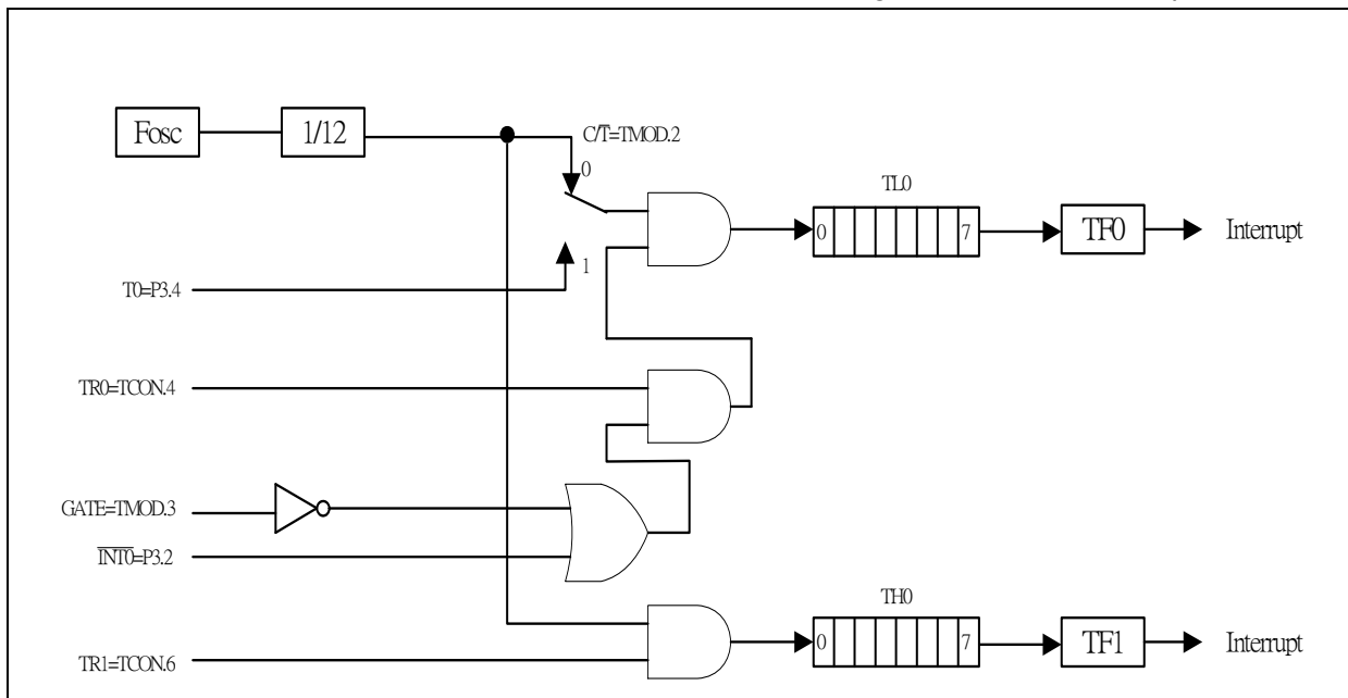
Figure 14-3 Timer/Counter Mode 3
