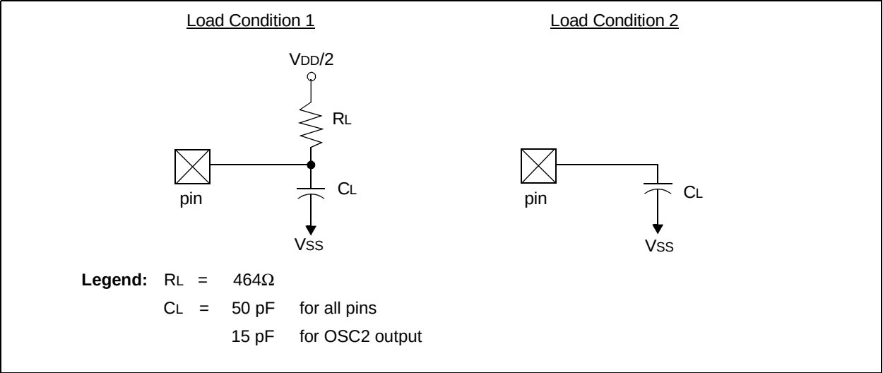
FIGURE 15-2: LOAD CONDITIONS
