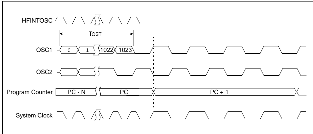
FIGURE 3-7: TWO-SPEED START-UP
