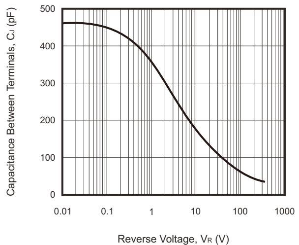
Fig.4 - Capacitance Characteristics
