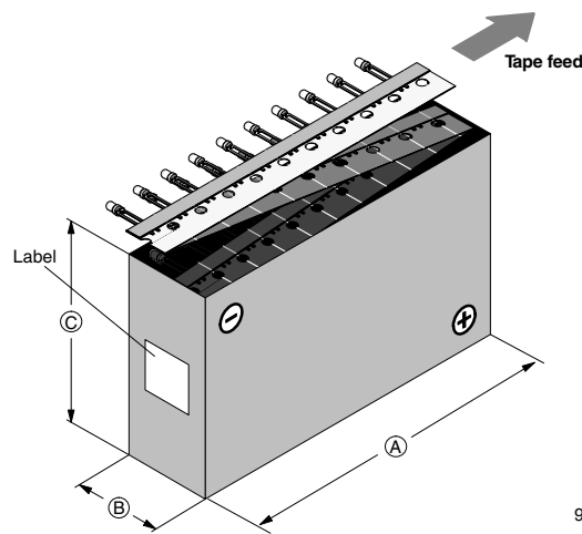
Fig. 19 - Tape Direction
