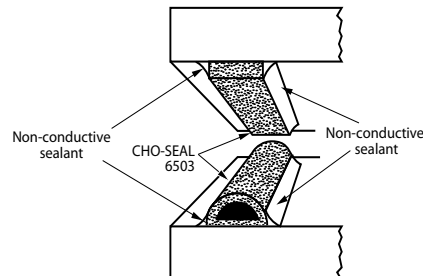
Figure 2-3. “Seal-to-seal” design incorporating CHO-SEAL® 6503 conductive silver-aluminum fluorosilicone gaskets on both mating flange surfaces. Gaskets are bonded and edge sealed to prevent moisture from entering the gasket/flange area.
