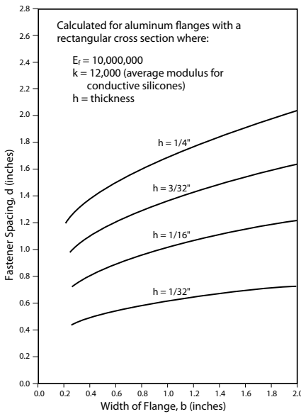
Figure 3-13. Fastener Spacing
