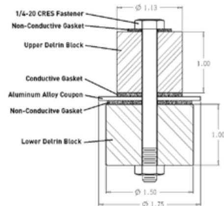
Figure 2-1 Test Fixture
