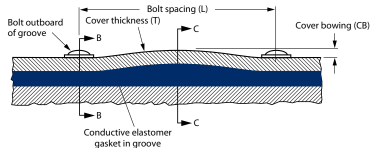
Figure 3-19. Section A-A of Assembled Enclosure Flange and Gasket (Sectioned midway through gasket and groove)
