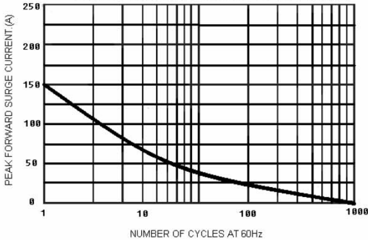
FIG.1-MAXIMUM NONO-REPETITIVE FORWARD SURGE CURRENT PER BRIDGE ELELEMENT
