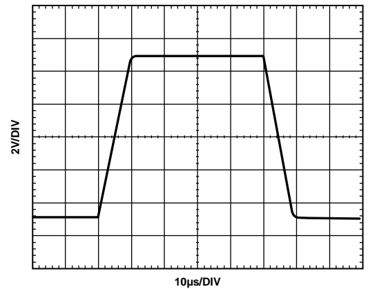
Figure 31. Large Signal Step Response
