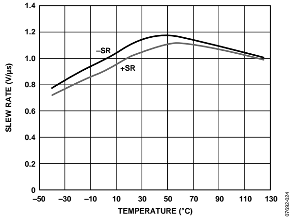
Figure 27. Slew Rate vs. Temperature, V_{IN} = 20 V p-p , 1 kHz
