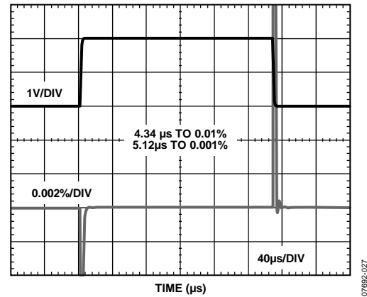
Figure 30. Large Signal Pulse Response and Settling Time, 2 V Step, V_S = 2.7 V
