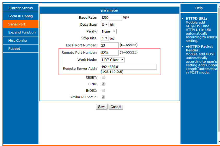
Figure 8 UDP Client
