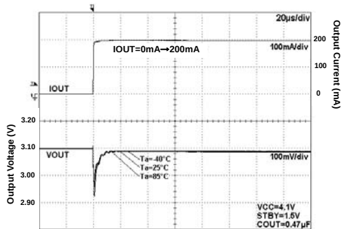
Fig 249. Load Response
