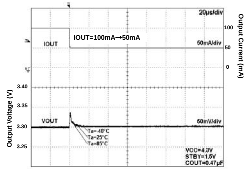
Fig 278. Load Response
