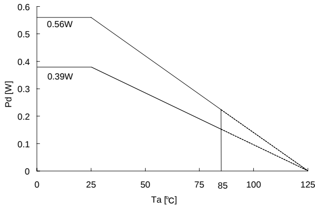
Fig. 285 SS0N004X1010 Power dissipation heat reduction characteristics (Reference)
