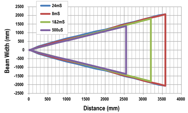
Figure 32. Opposed Mode—PIT66U
