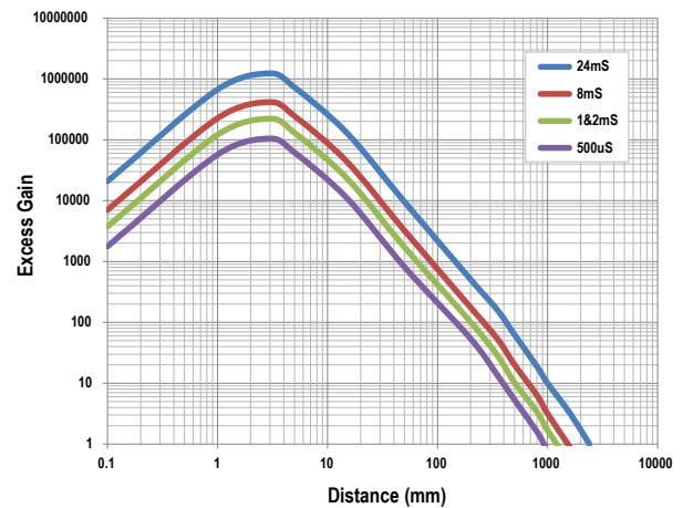
Figure 16. Diffuse—PBT66U
