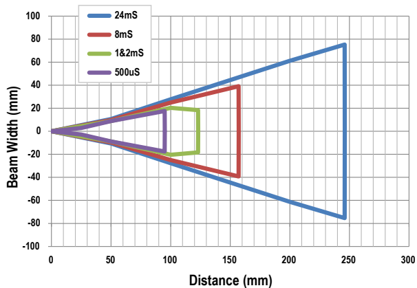
Figure 29. Opposed Mode—PIT16U
