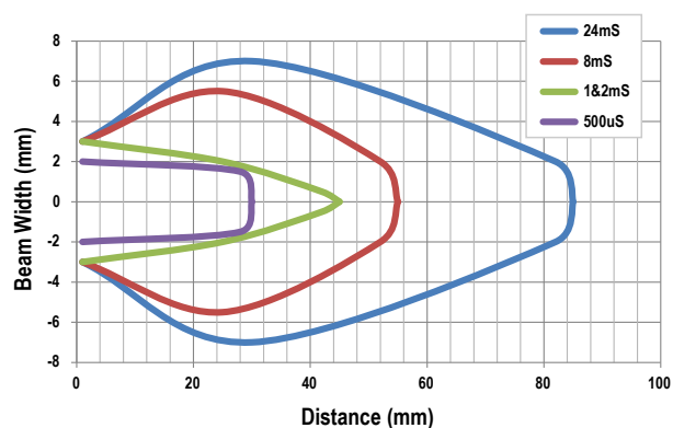
Figure 25. Diffuse—PBT16U
