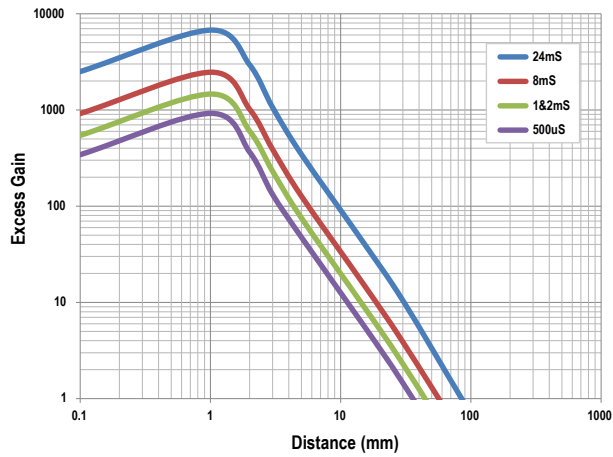
Figure 13. Diffuse—PBT16U
