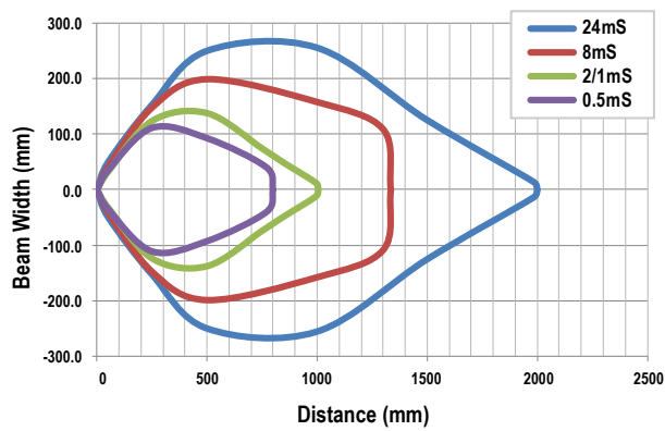
Figure 31. Opposed Mode—PIT46U
