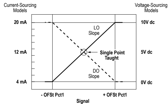
Figure 5. One-Point SET (Light Operate shown)
