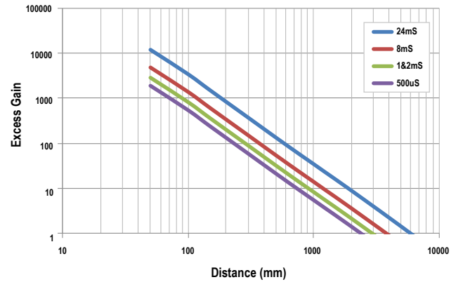
Figure 20. Opposed Mode—PIT66U
