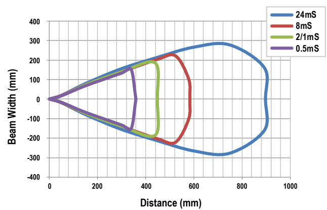
Figure 36. Opposed Mode—LIR1450
