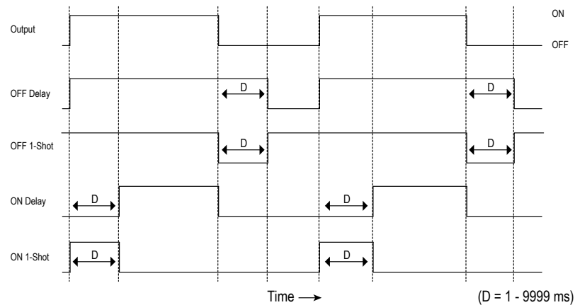
Figure 2. DF-G3 Delays/Timers
