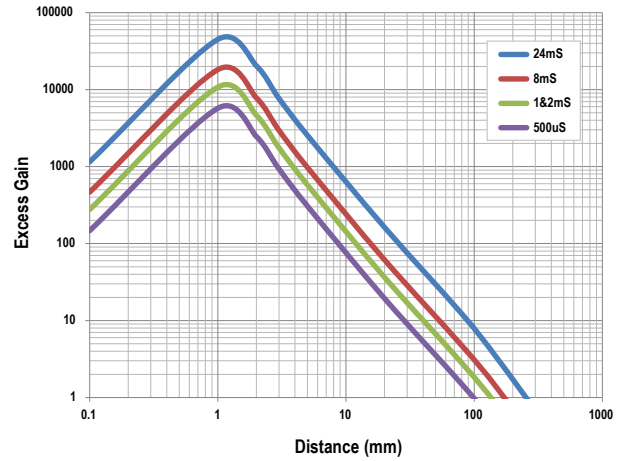
Figure 14. Diffuse—PBT26U
