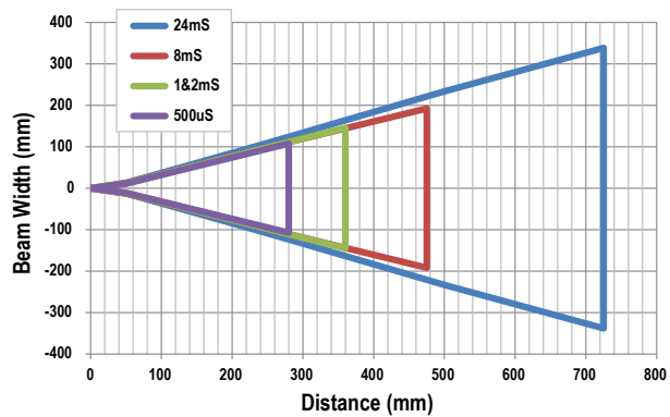
Figure 30. Opposed Mode—PIT26U
