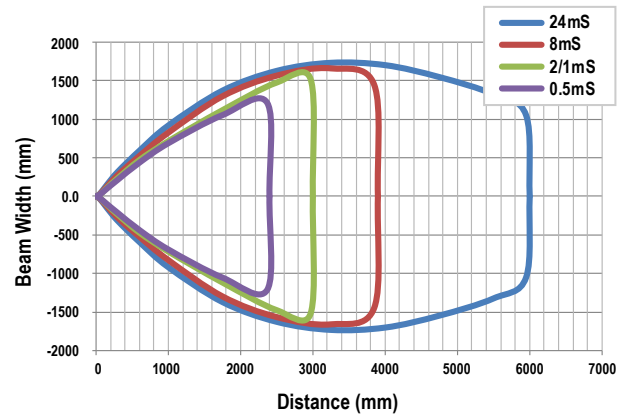
Figure 32. Opposed Mode—PIT66U
