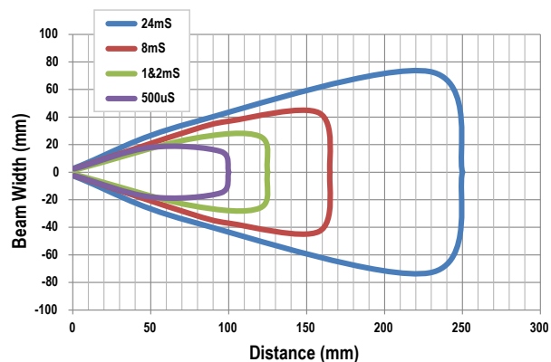
Figure 26. Diffuse—PBT26U
