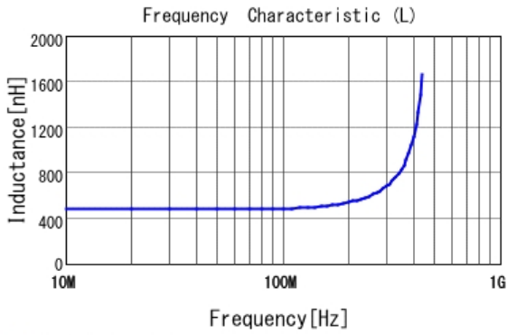
■ LQW2BASR47J00 L
