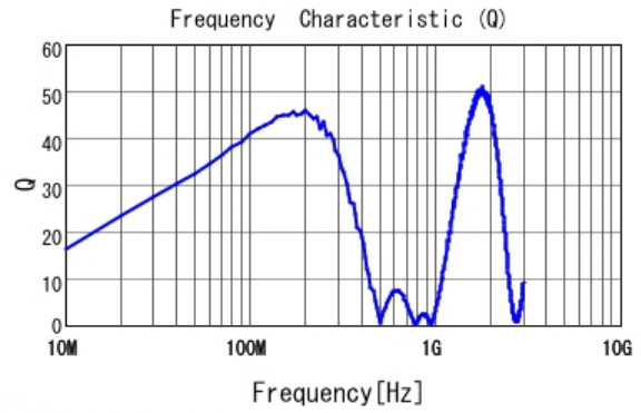
■ LQW2BASR47J00 Q
