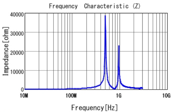
■ LQW2BASR47J00 |Z|
