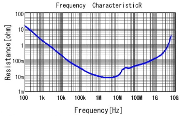
■ GRM188R71A684KA61 R DCOV, 25degC
