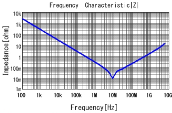
■ GRM188R71A684KA61 |Z| DCOV, 25degC
