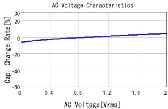
■ GRM188R71A684KA61 C-AC Voltage capchange, DCOV, 25.0d
