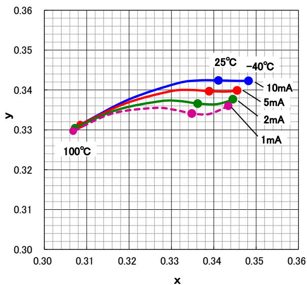
Ambient temperature vs. Chromaticity Coordinates
