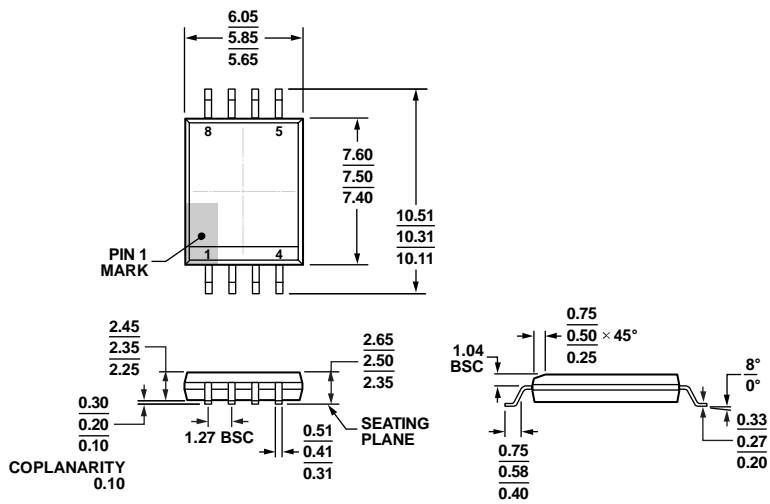
Figure 47. 8-Lead Standard Small Outline Package, with Increased Creepage [SOIC_IC] Wide Body (RI-8-1) Dimensions shown in millimeters
