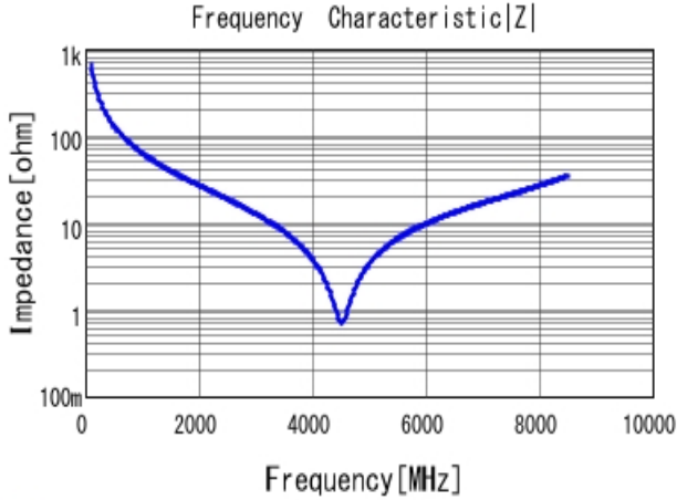
■ GRM1885C1H2R4CA01 |Z| DC0V, 25degC
