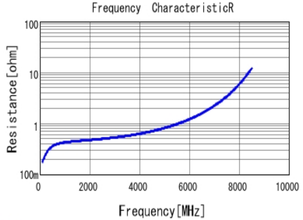
■ GRM1885C1H2R4CA01 R DC0V, 25degC
