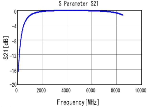
■ GRM1885C1H2R4CA01 S21 DCOV, 25degC
