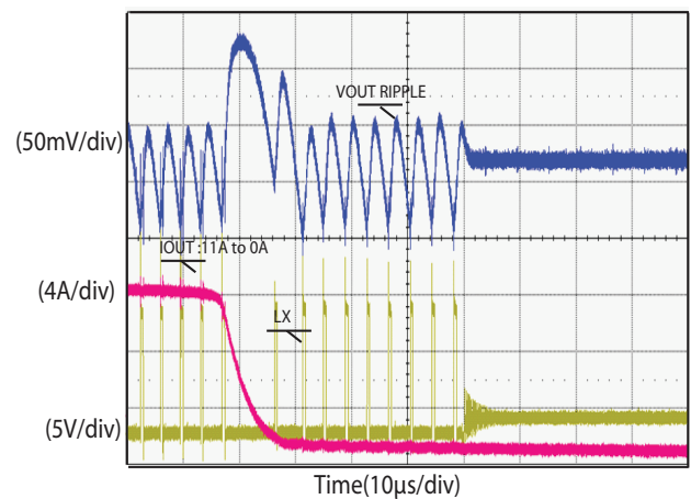
Transient Response - P-Save Load Falling (V_{DD} = 5\text{ V}, V_{IN} = 12\text{ V}, V_{OUT} = 1.5\text{ V}, I_{OUT} = 11\text{ A to } 0\text{ A}, \text{SiC401B}, dI/dt = 1\text{ A}/\mu\text{s})
