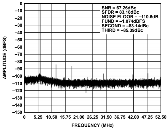
Figure 36. Single Tone Distortion AD8352 Driving AD9445, Encode Clock at 105 MHz with f_c at 100 MHz ( A_v = 10 dB), See Figure 34
