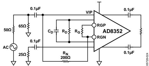
Figure 26. Single-Ended Schematic
