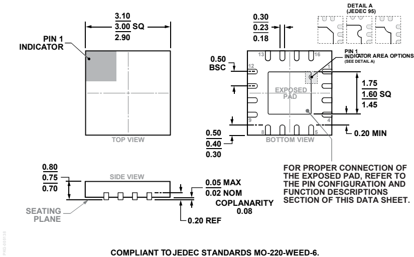
Figure 41. 16-Lead Lead Frame Chip Scale Package [LFCS] 3 mm × 3 mm Body and 0.75 mm Package Height (CP-16-22) Dimensions shown in millimeters
