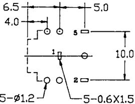
5- \phi 1.2 5-0.6X1.5 PCB LAYOUT (BOTTOM VIEW)
