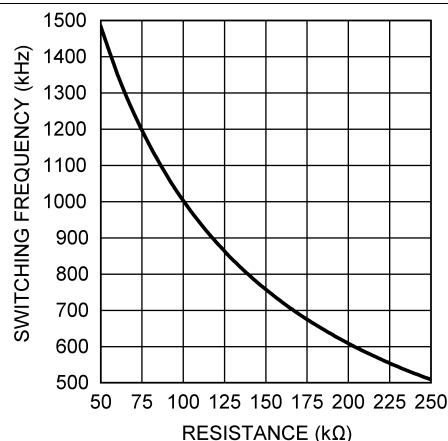
Figure 14. Switching Frequency vs R_T
