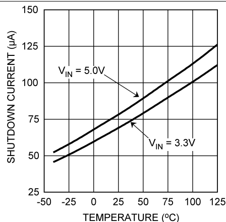
Figure 16. Shutdown Current vs Temperature
