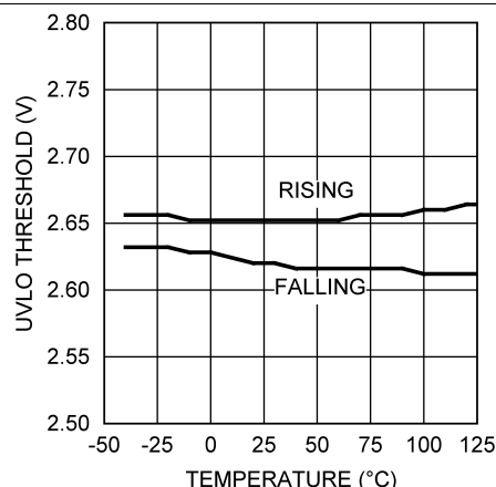
Figure 18. UVLO Threshold vs Temperature
