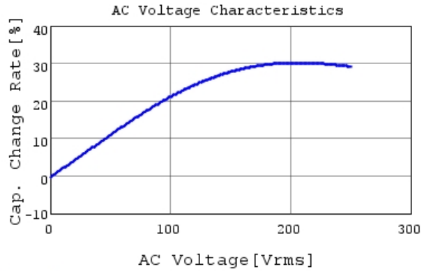
DE2E3SA222MA3BT02F C-AC Voltage capchange, I
