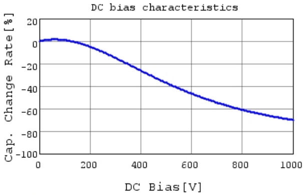
DE2E3SA222MA3BT02F C-DC bias capchange, 20.0
