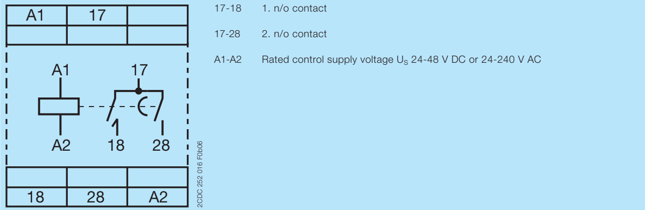
Connection diagram
