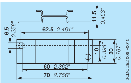
ADP.01 - Adapter for screw mounting
