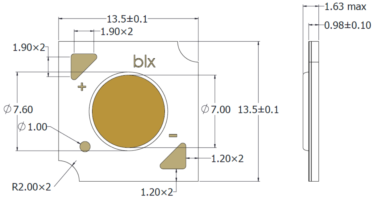
Figure 14: Drawing for V6 HD LED Array
