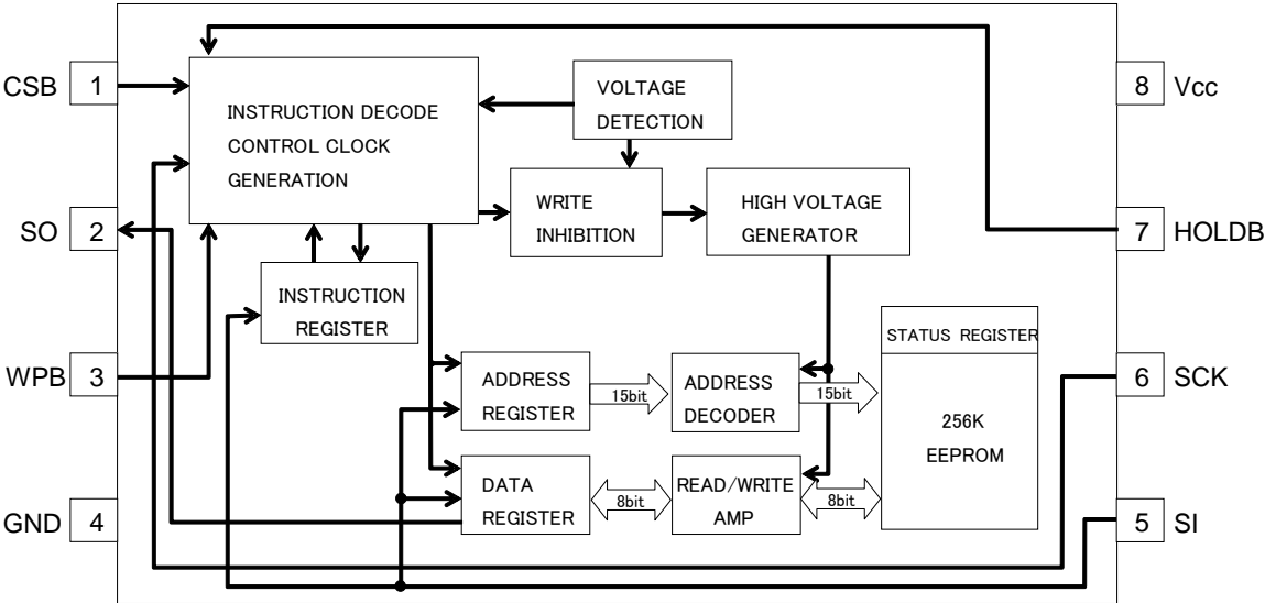
Figure 3. Block Diagram
