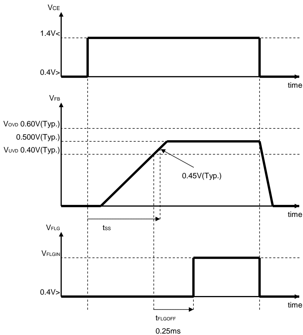
Fig. 2 Flag Function Sequence
