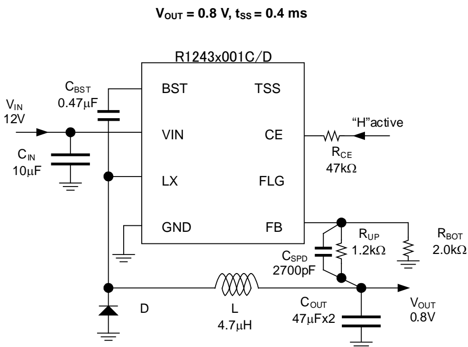
R1243x001C/D Typical Application
