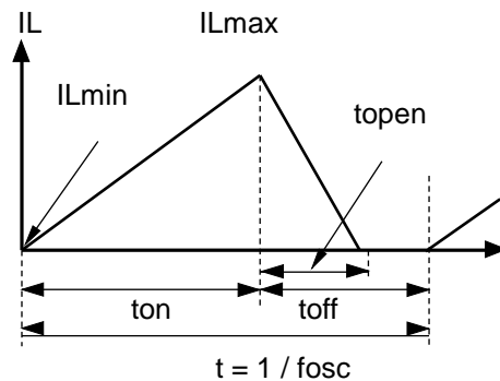
Inductor Current flowing through Inductor
