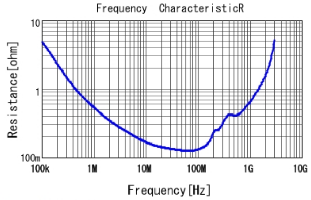
GCJ31BR73A472KXJ1 R DCOV, 25degC
