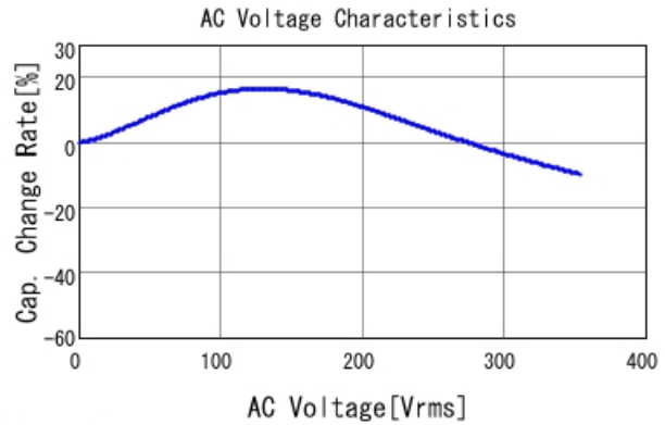
GCJ31BR73A472KXJ1 C-AC Voltage capchange, DCOV, 25
