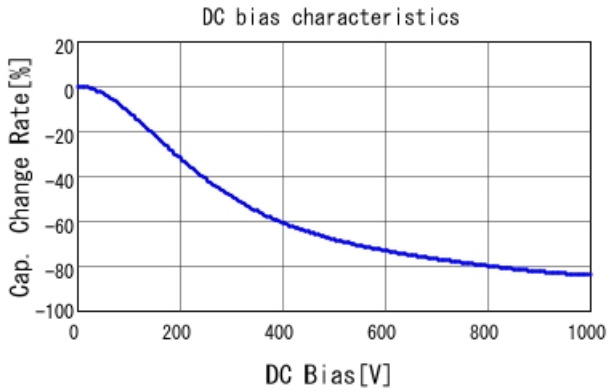
GCJ31BR73A472KXJ1 C-DC bias capchange, 25.0degC, A
