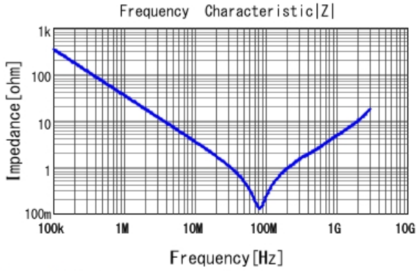
GCJ31BR73A472KXJ1 |Z| DCOV, 25degC
