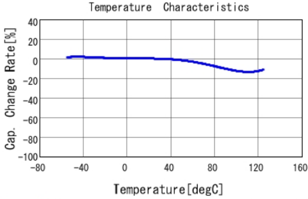
GCJ31BR73A472KXJ1 C-Temp. capchange, DCOV, AC1Vrms
